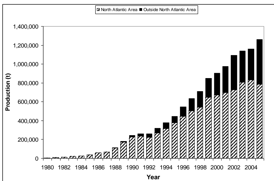
Figure 2.2.1. World-wide production of farmed Atlantic salmon, 1980–2005.
