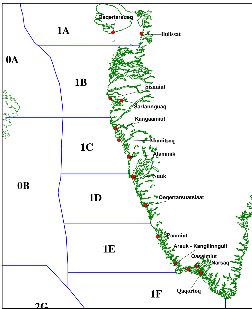
Figure 5.9.1.1. West Greenland NAFO divisions.
