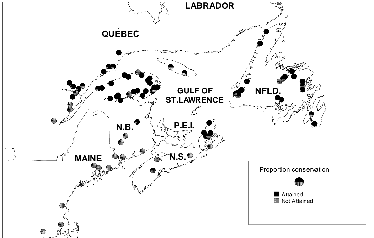
Figure 4.9.2.4. Proportion of the conservation requirement attained in assessed rivers of the North American Commission in 2005.
