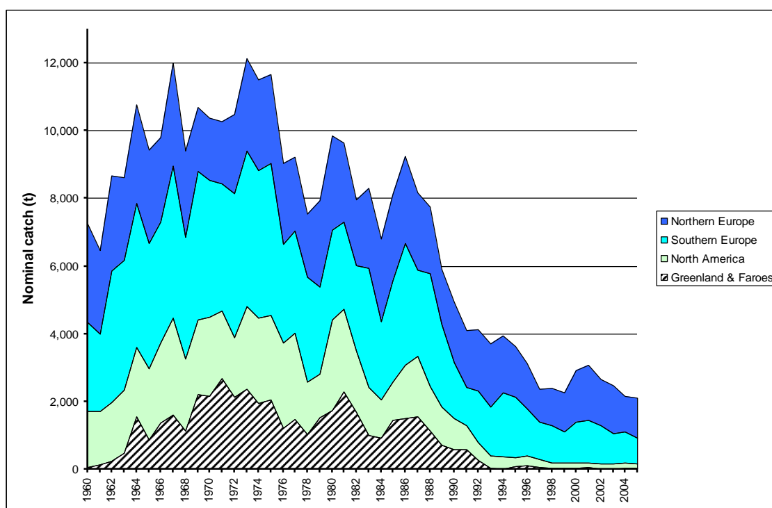
Figure 2.1.1.1. Nominal catches of salmon (tonnes round fresh weight) in four North Atlantic regions, 1960-2005.
