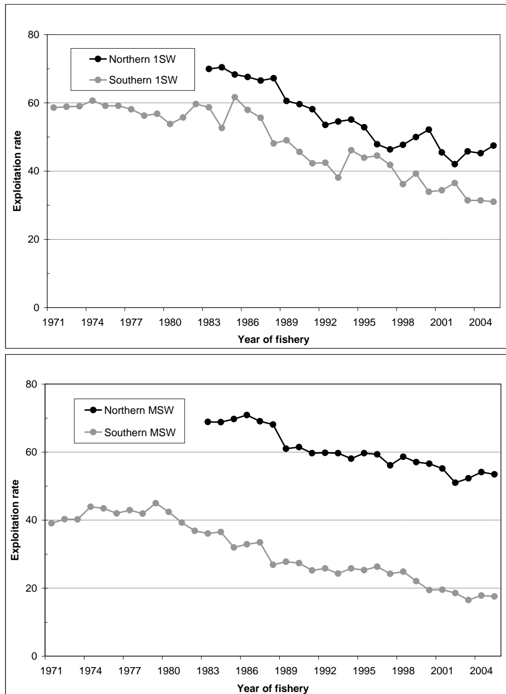
Figure 3.1.2. Estimated mean exploitation rates (1971–2005) for Northern and Southern European 1SW and MSW stocks.
