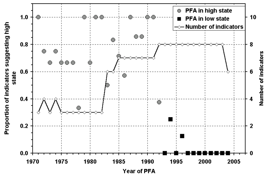
Figure 2.6.3. Assigning the state of PFA abundance for the years 1971 to 2004 using the returns of large/2SW salmon simultaneously for three to eight monitored rivers in North America.
