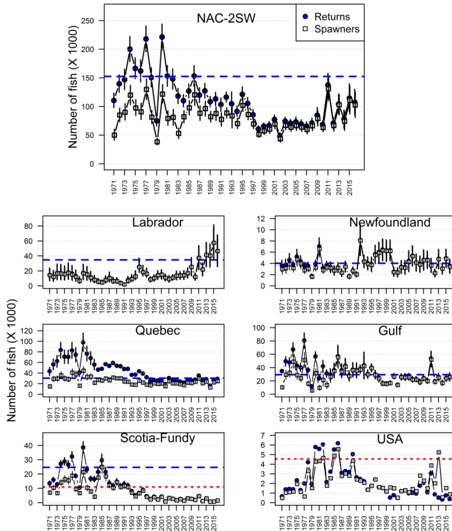
Figure 8 Estimated (median, 5th to 95th percentile range) returns (shaded circles) and spawners (open squares) of 2SW salmon, for eastern North America overall (top panel) and for each of the six regions. The blue dashed line is the corresponding 2SW CL; the 2SW CL (29 199 fish) is off the scale in the plot for USA. The red dotted lines in the Scotia–Fundy and USA panels are the region-specific management objectives. For USA, estimated spawners exceed the estimated returns in some years because of adult stocking restoration efforts.
