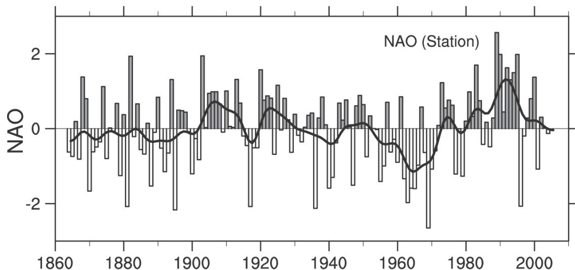
Figure 20 Normalized indices (units of standard deviation) of the mean winter (December–March) NAO developed from sea level pressure data. The index is based on the difference of normalized sea level pressure between Lisbon, Portugal and Stykkisholmur/Reykjavik, Iceland from 1864 to 2005. The average winter sea level pressure data at each station were normalized by dividing each seasonal pressure anomaly by the long-term (1864 to 1983) standard deviation. The smooth black curves show decadal variations (see Appendix 3.A of IPCC, 2007). The individual bar corresponds to the January of the winter season (e.g., 1990 is the winter of 1989/1990). Updated from Hurrell et al. (2003); see http://www.cgd.ucar.edu/cas/jhurrell/indices.html for updated time-series. (Source: Top panel Figure 3.31 from IPCC, 2007).
